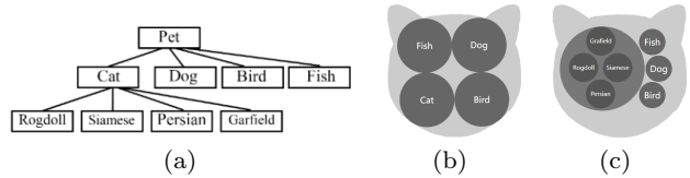
Fig. 4: (a) tree structure of menu, (b) layout of node “Pet” and (c) layout of node “Cat”.
