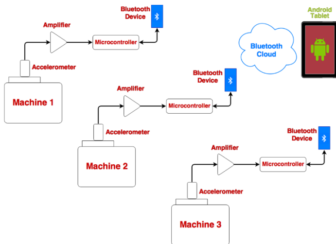
Fig. 3 Proposed architecture.
