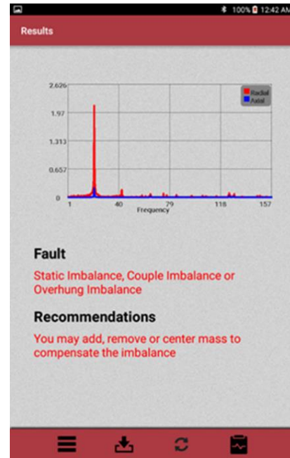
Fig. 10. Mass unbalance at 1254 rpm.
