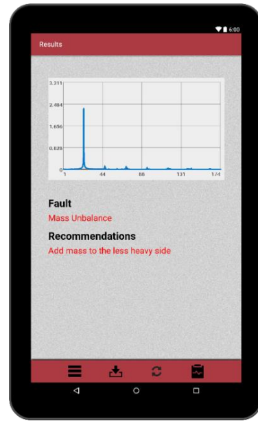
Fig. 6 Unbalance diagnosis
