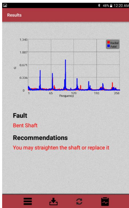
Fig. 11. Bent shaft at 1676 rpm.
