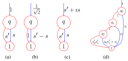
Fig. 3. symTDD representations of (a) a 1-qubit symbolised computational basis state |s\rangle ; (b) H|s\rangle ; (c) R_2|s\rangle ; (d) the output state of the 2-qubit Grover oracle applied on |001\rangle , where |1\rangle is the state of the ancilla qubit.
