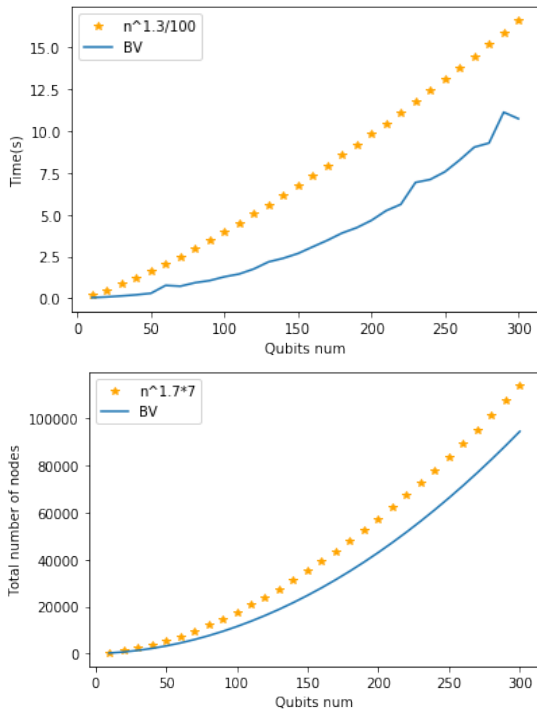
Fig. 8. The time and space consumption of using symTDDs to verify the Bernstein-Vazirani algorithm. In the figure, we use \hat{n} to represent the exponent and n^{1.3}/100 , n^{1.7*7} represent n^{1.3}/100 and 7n^{1.7} respectively.
