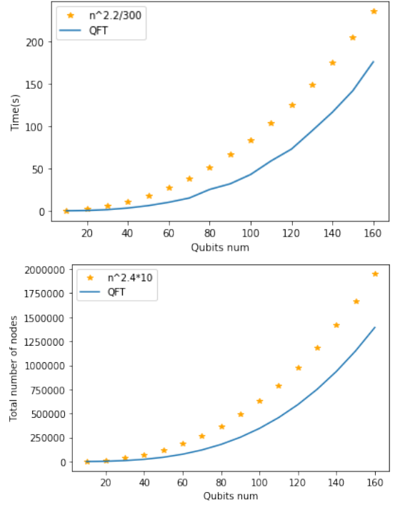
Fig. 6. The time and space consumption of symTDD execution of 10-160 qubits QFT circuits. In this figure, we use \hat{\cdot} to represent the exponent and n^{\cdot} n^{2.2/300} , n^{\cdot} 2.4 \cdot 10 represent n^{2.2}/300 and 10n^{2.4} respectively.
