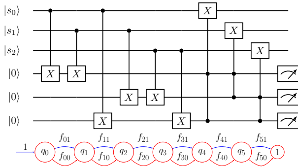
Fig. 10. The circuit (top) and the symTDD (bottom) for verification of the bit-flip code circuit. Principle of deferred measurement [8] is used.
