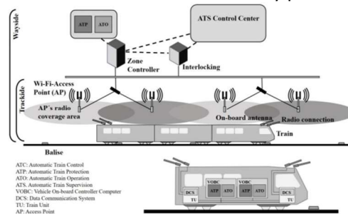
Figure 3: CBTC (Communication Based Train Control) equipment (From WIT Press)
