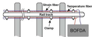
Figure 8: Temperature and track tension/pressure control (from ScienceDirect.com)
