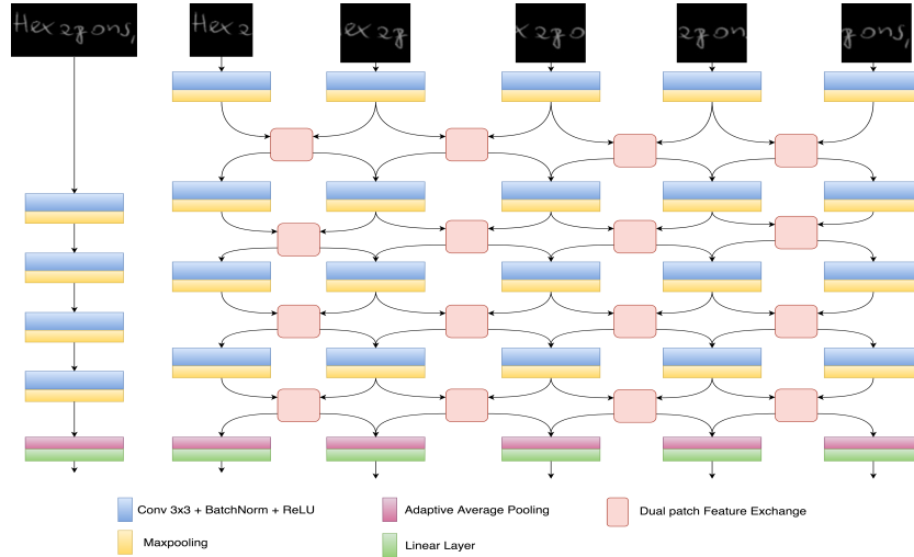
Fig. 4: Architecture of our proposed PatchNet
