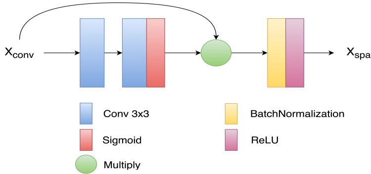
Fig. 1: Architecture of Spatial attention unit employed in SA-Net
