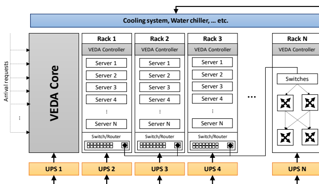
Fig. 4. A simplified data center and related components as well as the location of VEDA framework
